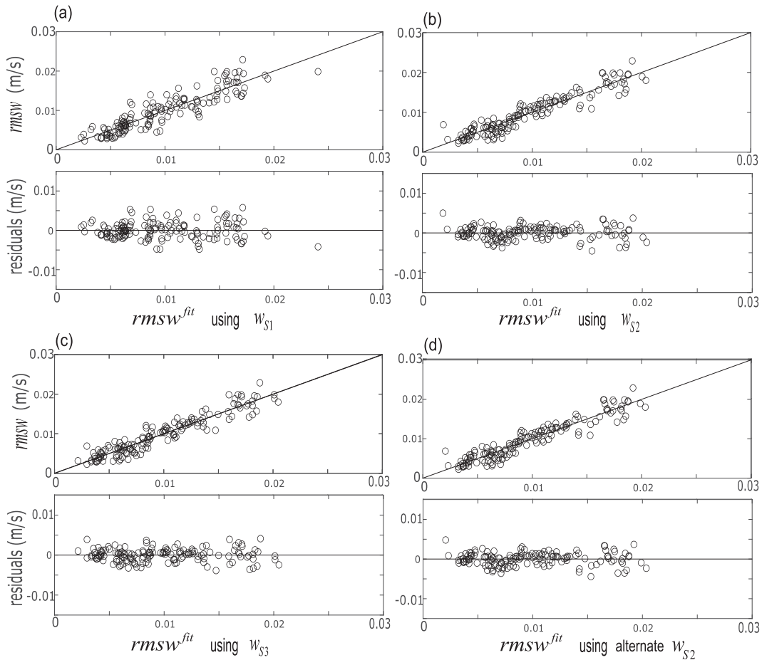
FIG. 3. The upper panels in each group show values of rmsw observed at LEO as a function of values predicted using observational values of w_* and either (a) w_{S1} = u_* , (b) w_{S2} = (u_* U_S)^{1/2} , or (c) w_{S3} = (u_*^2 U_S)^{1/3} , with the latter two calculated using the near-surface-integral value U_S = \text{int}U_{S3} . The solid line is a 1/1 relationship, a line with slope 1 through the origin. The lower panels in each group show the associated residuals ( \text{rmsw} - \text{rmsw}^{\text{fit}} ). (d) For comparison with (c), results for the alternate fit using w_{S2} calculated with the LEO surface-layer value of U_S = U_{SL} = \text{int}U_{S3} - u_{\text{ref}}^S .
